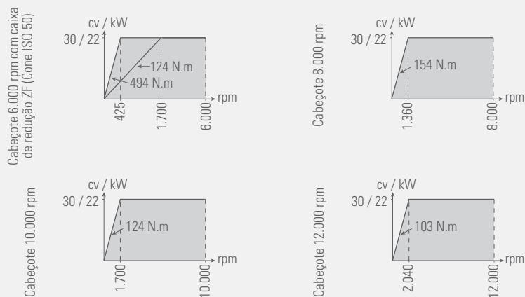
ROMI D 1500 - CNC Siemens 828D (regime S6 - 60% - 10 min)
