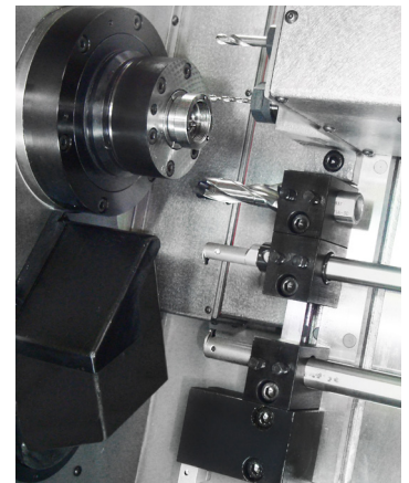
Furar e rosquear axial
